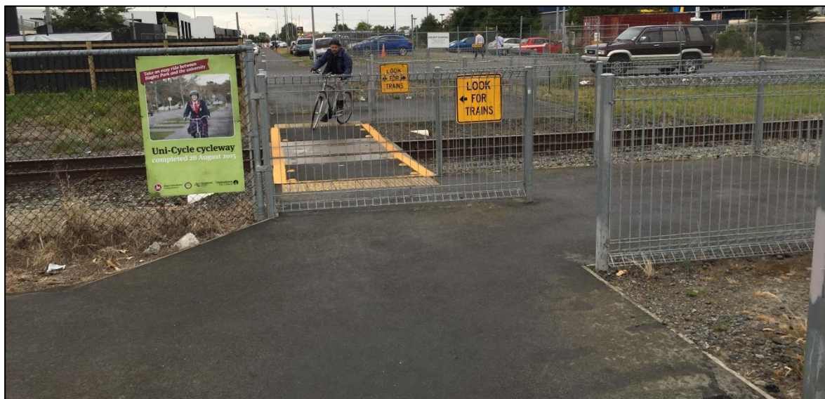
Figure 61: Level crossing with maze approaches and warning signs, Christchurch
