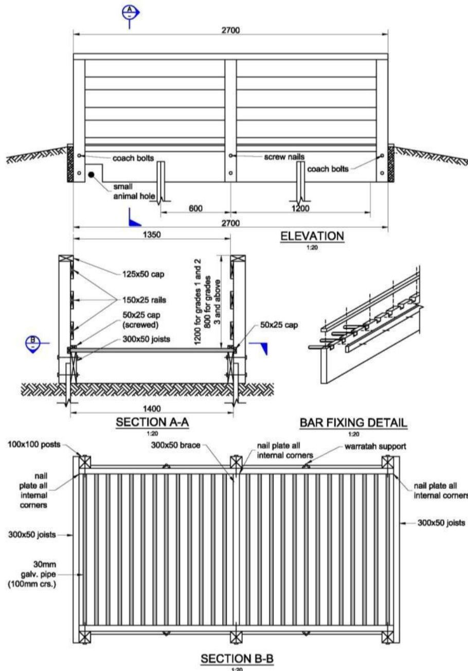
Figure 51: Cattle stop design – plan view (adapted from Christchurch City Council designs)
