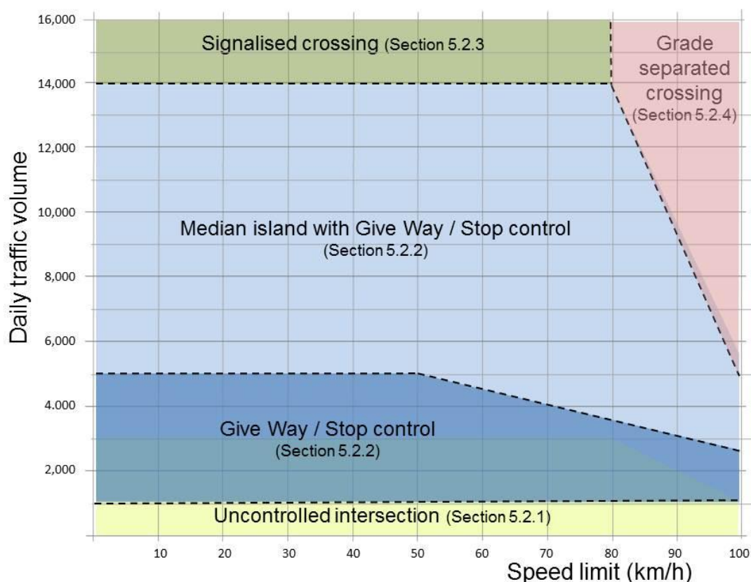
Figure 39: Crossing types
