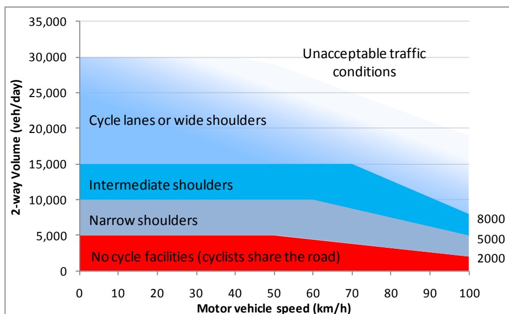
Figure 32: Trail type for Grade 5 on-road trails
