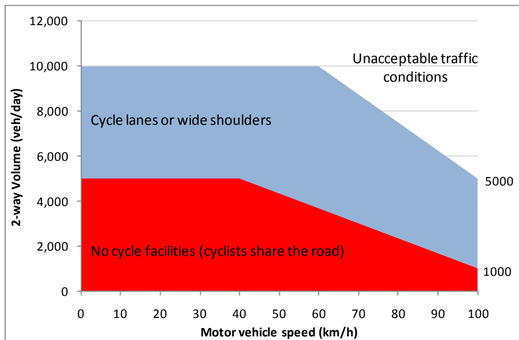
Figure 31: Trail type for Grade 3 and 4 on-road trails
