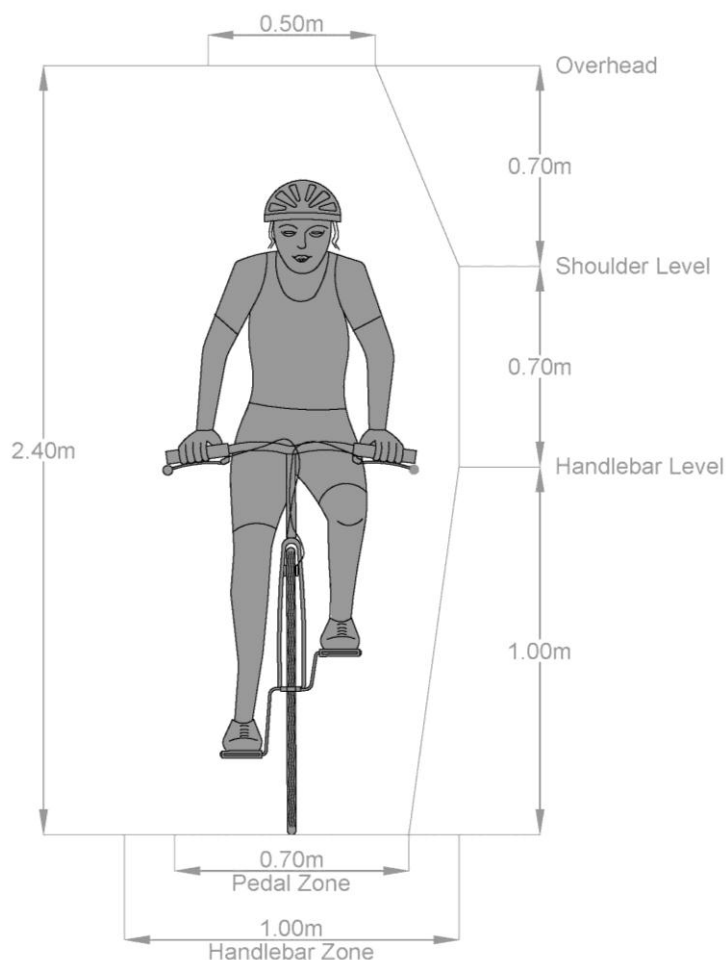
Figure 17: Bicycle operating space
