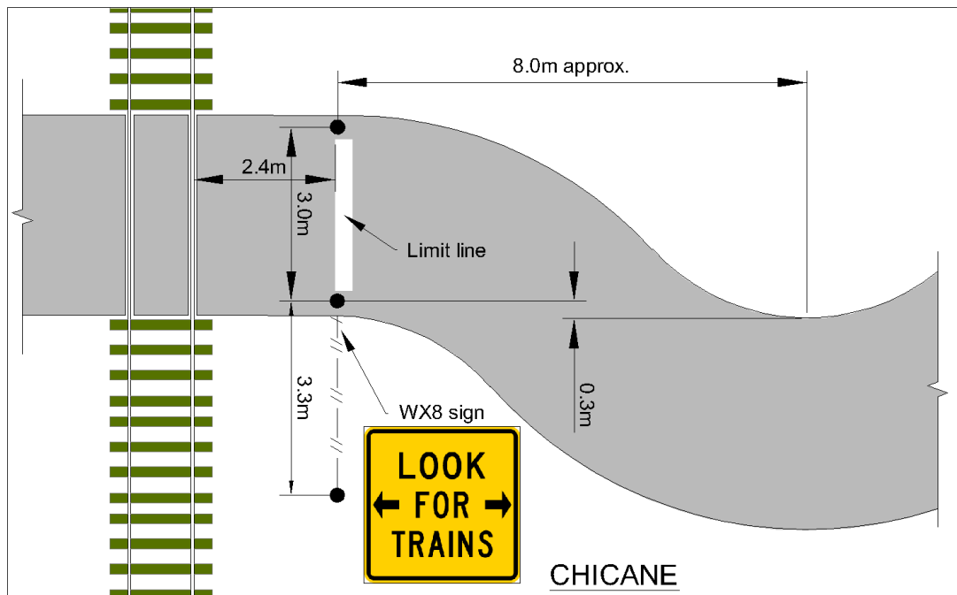
Figure 43: Chicane design; slows cyclists before crossing railway line
