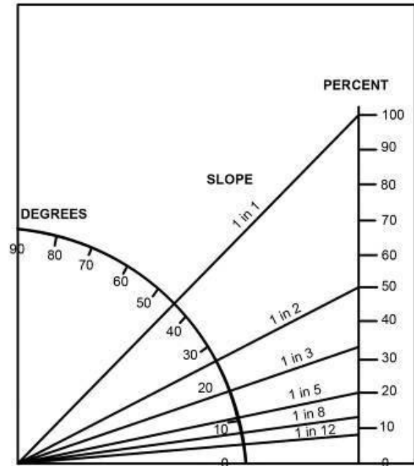
Figure 14: Relationship between degrees, percent and slope
