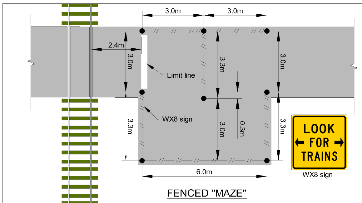
Figure 44: Fenced maze design; slows cyclists before crossing railway line
