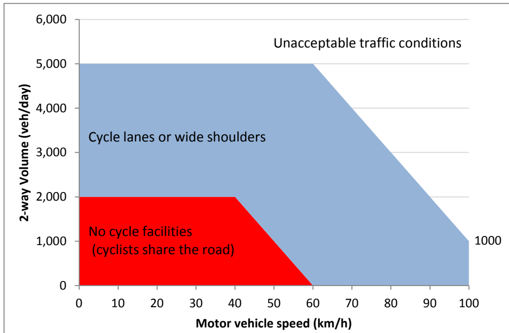
Figure 30: Trail type for Grade 1 and 2 on-road trails
